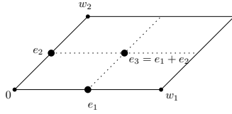
Figure 3.2: The 2-torsion points of E_\Lambda
